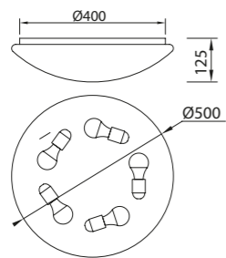
5410 Blanco-White 5L x E27 máx. 20W LED
